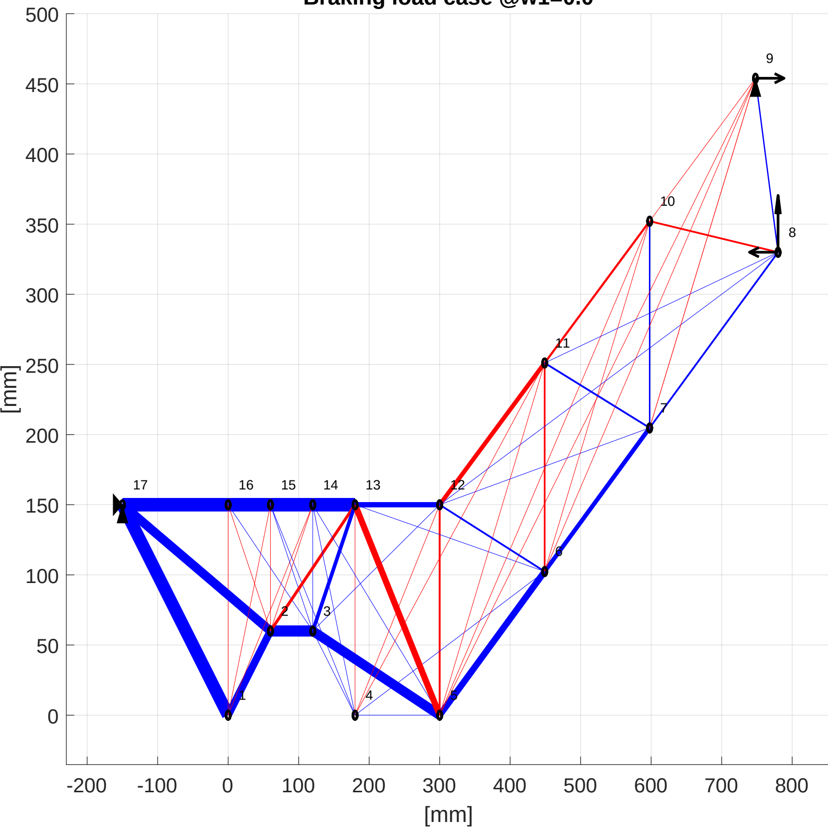
Braking load case @w1=0.0
