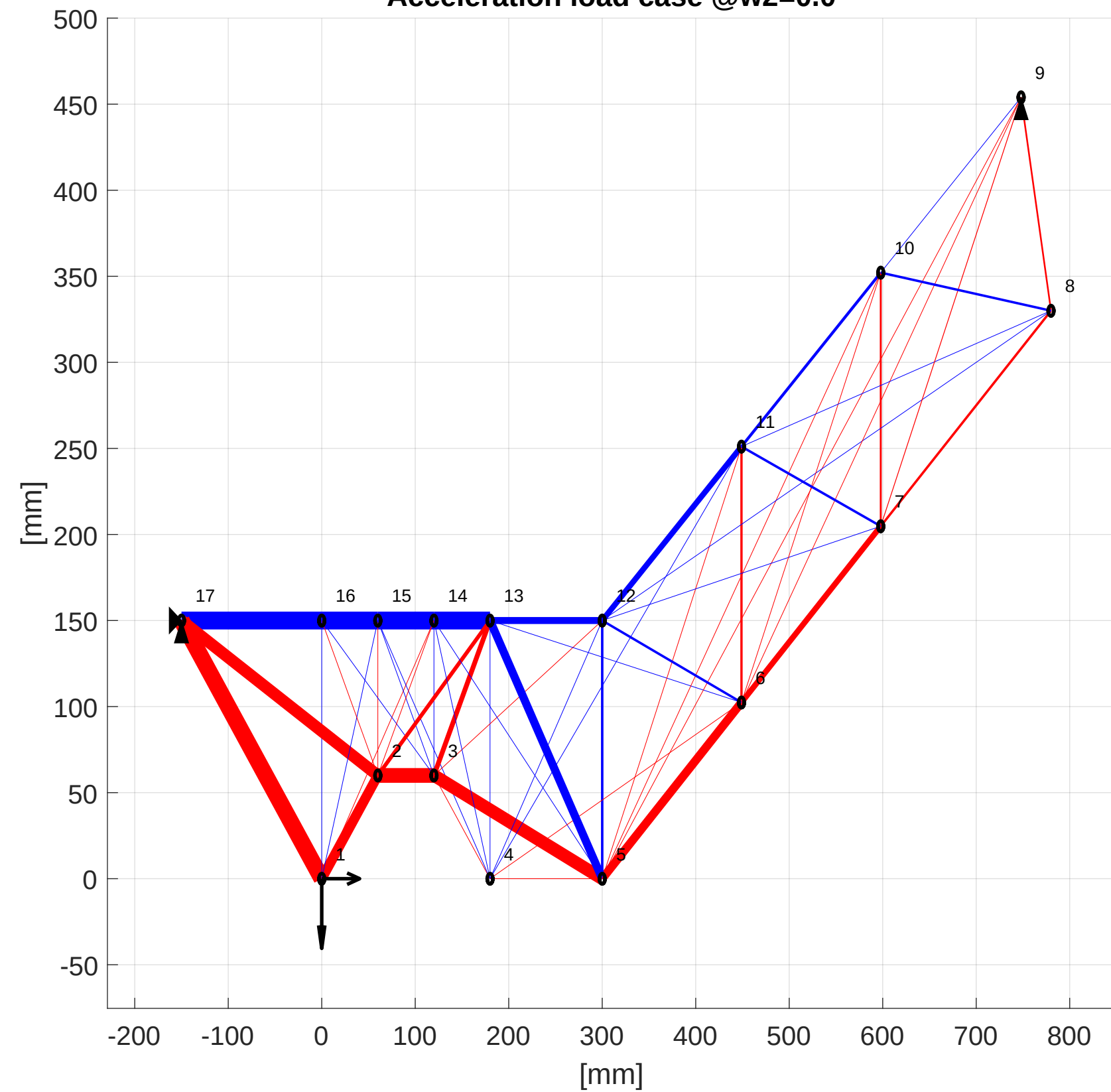
Acceleration load case @w2=0.0
